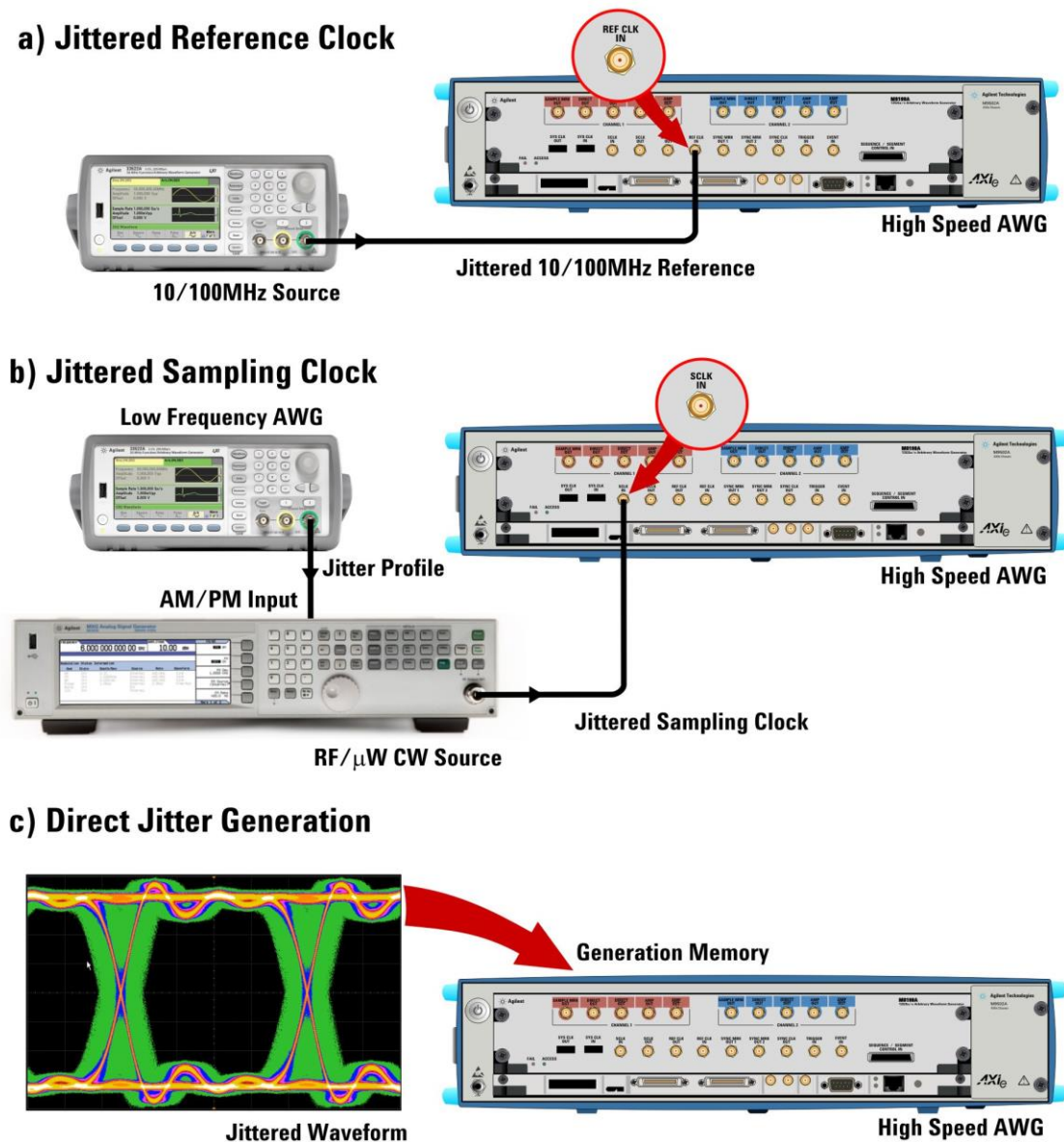
Figure 75: There are several ways to generate jittered waveforms. For relatively low-frequency jitter, a jittered reference clock may be used (a). Jitter will be transferred to the output signal through a PLL oscillator so its jitter transfer response must be calibrated. Some AWGs incorporate external sampling clock inputs. A jittered sampling clock will result in a jittered waveform (b). The most flexible way to generate jitter is by calculating an already jittered waveform and generate it directly at a fixed sampling rate (c).
