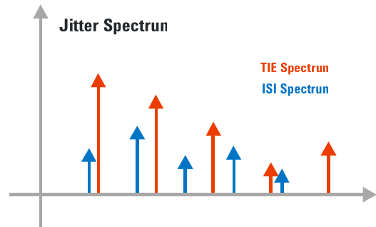
Figure 77: Direct Jitter generation may result in unexpected jitter behavior. For looping signals, all synthesized jitter components will be periodic. In (a) periodic jitter (sinusoidal in this example) is mistaken as data dependent jitter because there is a perfect correlation between data and jitter in both time and frequency domains. In (b) sinusoidal jitter is reported as periodic jitter while the data dependent jitter profile shows a small amount of ISI caused jitter. In this case, the same data sequence is repeated within the waveform memory while the sinusoidal jitter frequency has no direct harmonic relationship with it.
