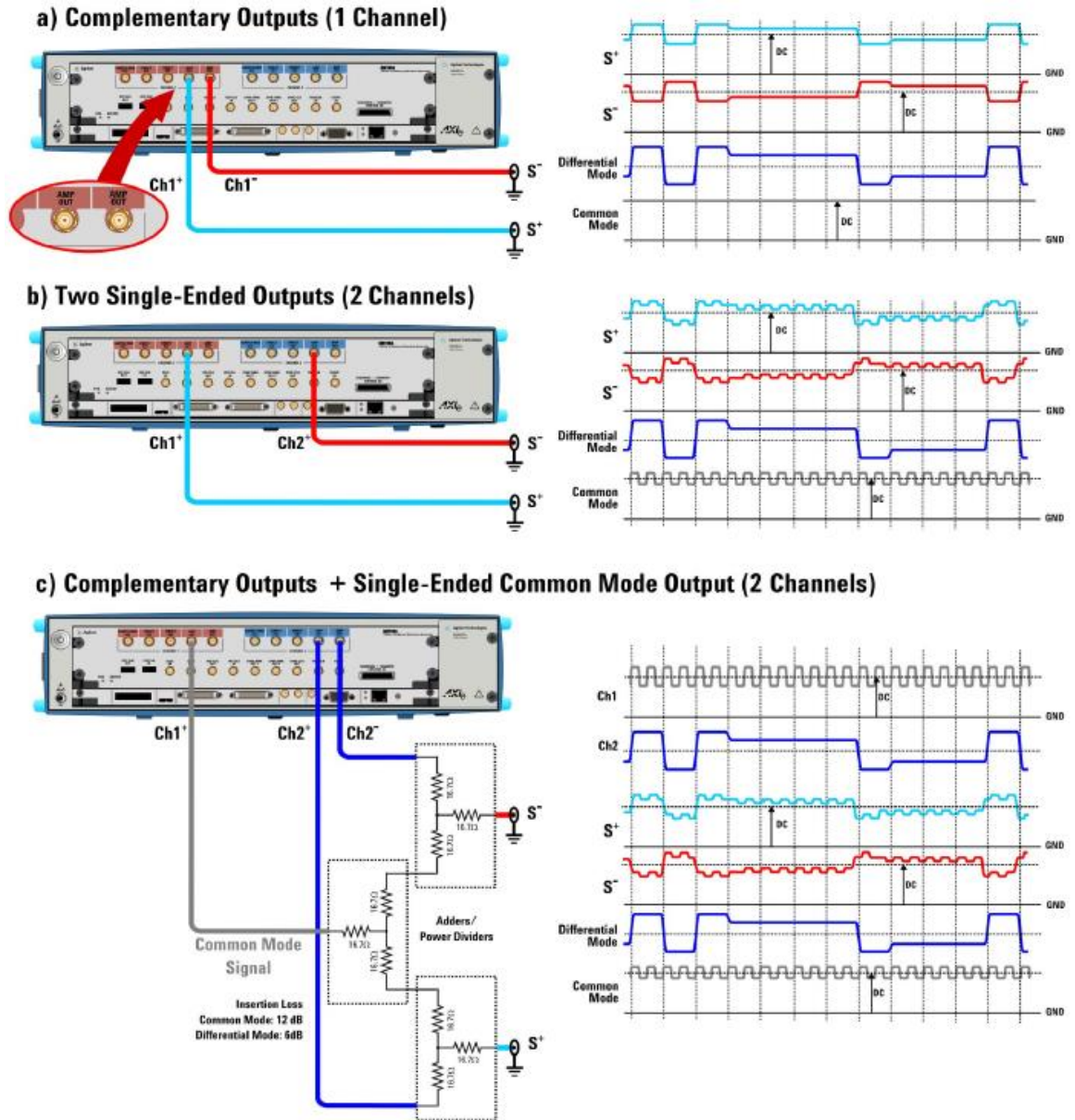
Figure 80: There are several ways to generate differential signals with a AWG other than a single-ended to differential converter. Most high-performance arbs incorporate a complementary output where the DC level can be set-up independently (a). Using two independent channels allows for full differential connection emulation (b) as any combination of common mode and differential mode signals may be implemented. Combining complementary output and single-ended channels can offer the same results. Combining the signals, though, may result in lower amplitude differential pairs.
