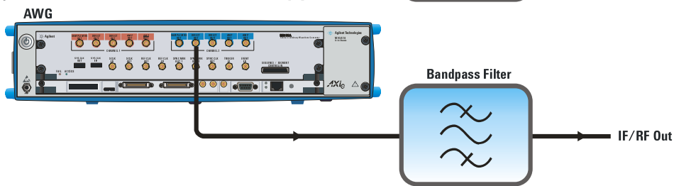
Figure 85: AWGs can generate RF signals in different ways. Traditional vector signal generation (a) relies on two-channel AWGs to generate quadrature baseband signals ( I and Q ). Modern high-speed AWGs can directly generate one or multiple dissimilar modulated carriers (b) right at the target RF frequency or at a useful intermediate frequency (IF). It is possible to reach even higher carrier frequencies by using the signal image in the second Nyquist band (c). The doublet mode introduced by the M8190A 12 GSa/s is especially adequate for this kind of operation.
