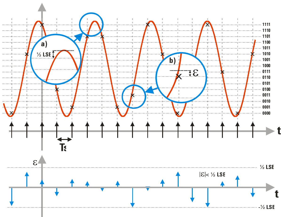
Figure 21: Quantization error can be analyzed as a sampled waveform itself. The resulting quantization noise waveform \epsilon(N T_s) is bounded to \pm 1/2 \text{ LSE} and the amplitude distribution uniformly over the whole range. Amplitude of the input waveform can go beyond 1/2 \text{ LSE} (a) and still keep the bounded error criteria (b).
