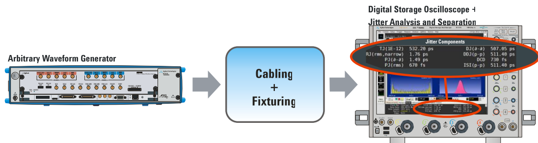
Figure 78: Jitter calibration must be used to compensate the effects of the AWG's intrinsic jitter and other sources such as cabling and fixturing. Without calibration random and data dependent jitter (especially ISI) would be higher than expected affecting the accuracy of any jitter tolerance test. Proper jitter calibration requires a low jitter noise floor analysis instrument and some jitter analysis software capable of doing jitter component separation.
