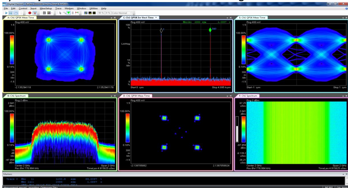
Figure 100: Incorrect wrap-around handling results in highly distorted signals when the signal is looped for continuous generation (b). Distortions show-up at all domains: time (see eye diagram), frequency (see spectral growth in the signal spectrum), and modulation (see constellation diagram). EVM spikes show up every occurrence of the signal. Properly synthesized signals (a), designed for continuous play-back, do not show any of these impairments and allow accurate measurements and glitch free operation of the DUT.
