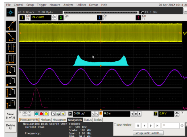
Figure 79: Then number of samples in an edge defines the timing control granularity. Here, the same sinusoidal jitter is applied to a binary sequence. With 0 samples in an edge (a) sinusoidal jitter is quantized (also visible in the jitter histogram) and its spectrum shows unwanted harmonics. One sample in an edge (b) results in a smoothed TIE waveform but it is still distorted. Setting up two samples per edge solves the distortion problem (c) as timing granularity is only limited by the vertical resolution.
