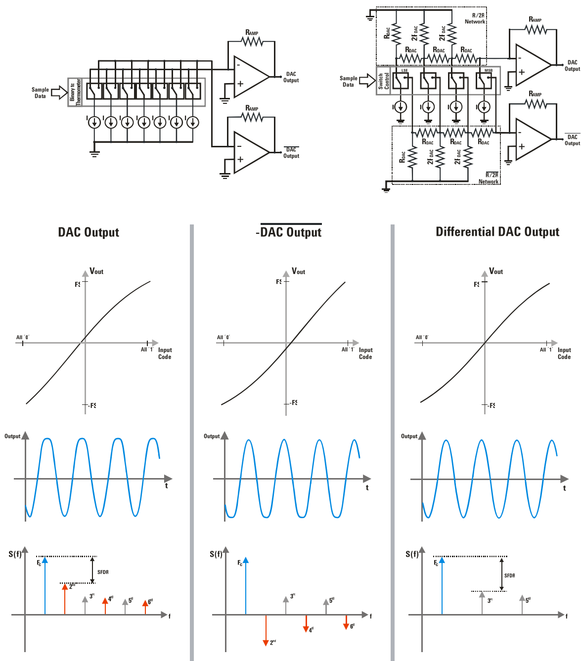
Figure 32: Complementary output DACs implement a differential output using a single set of current elements (current source + switch). Beyond the convenience of differential outputs, this strategy improves linearity as it cancels the asymmetrical component of the transfer function. Above, complementary output arrangements for a thermometer DAC (left) and an R/2R ladder DAC (right).
