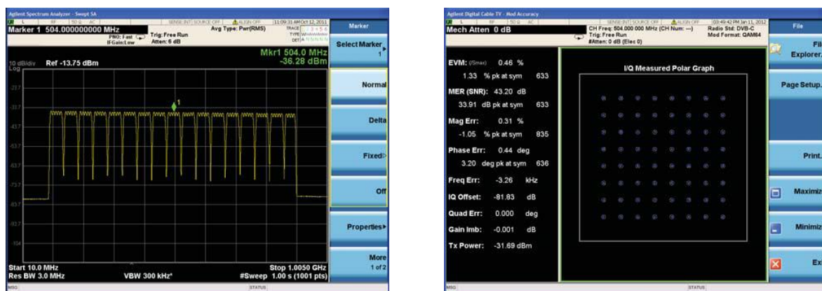
Figure 95: 84 64QAM DVB-C signals being generated simultaneously by an AWG (A Keysight M8190A). Notice the excellent available dynamic range and the lack of spurs (left) and the modulation quality obtained (right) with EVM lower than 0.5%.
