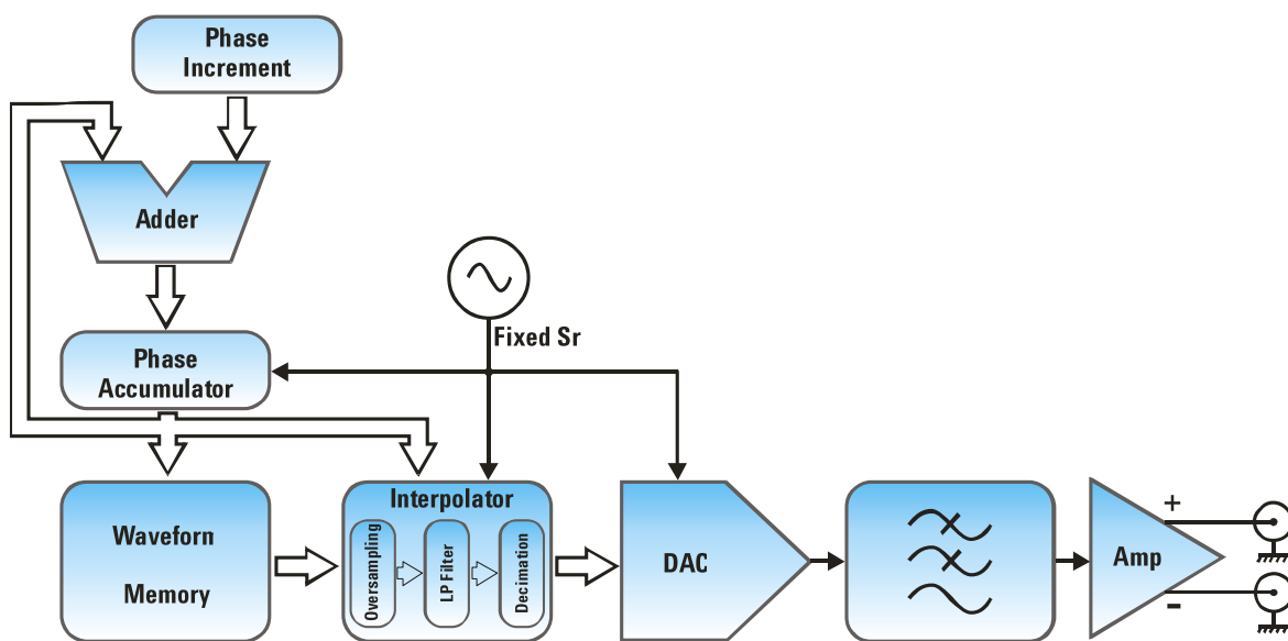
Figure 19: Block diagram for a (Trueform) architecture AWG
