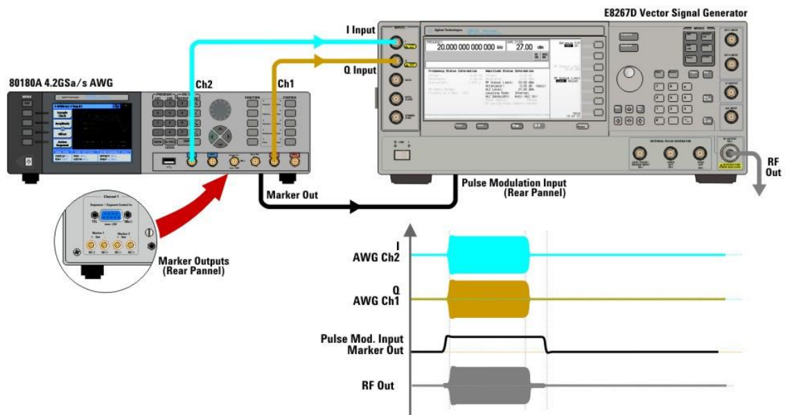
Figure 56: Controlling other instruments and/or the DUT is another application of markers. Here, one of the markers of an AWG is used to switch-off the RF output of a vector signal generator used to generate a pulsed RF signal while the same arb is generating the I and Q baseband signals through its two analog channels. Notice that even when the I and Q signals are not active, a remaining RF carrier is still present at the RF generator output. The Pulse modulation input controlled by the marker switches off the RF output improving the dynamic range of the RF signal.
