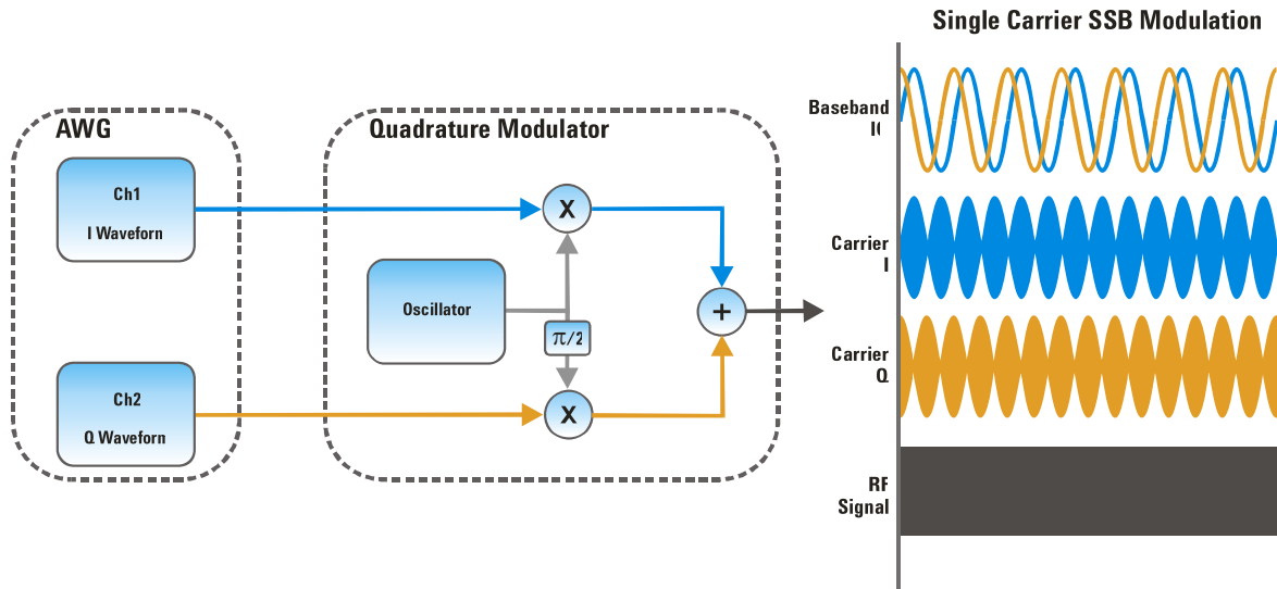
Figure 86: Quadrature modulation apply two basebands signals to carrier-suppressed AM modulators fed by two carriers of the same frequency and 90° phase difference. The orthogonality of the two carriers makes possible the transmission of two independent signals in the same frequency band. A perfect quadrature modulator produces a single carrier of f_c - f_m or f_c + f_m when two equal power sinusoidal signals of frequency f_m and 90° relative phase are applied. The resulting RF signal will be a single side band (SSB) carrier with constant amplitude envelope.
