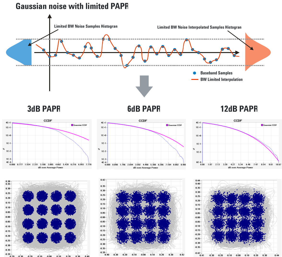
Figure 99: When synthesizing a signal with added Gaussian bandwidth-limited noise, clipping the signal to limit the effects of the noise crest factor is not an option. Clipping is a highly non-linear operation that results in signal distortion and spectral growth. Baseband noise samples, though, may be limited to some extreme values but, after applying a near-ideal bandwidth limited interpolator, the actual PAPR will grow significantly. Here, three different PAPR have been applied to the same baseband samples so the SNR is approximately the same for the 16QAM target signal. In some cases, there will be no errors caused by noise as the signal never goes beyond the decision thresholds. In this example, selecting the 12 dB PAPR will result in a very realistic noise behavior with a very little overall (signal + noise) peak-to-peak amplitude penalty.
