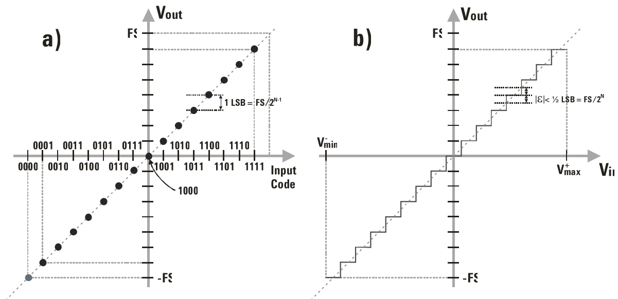
Figure 20: Transfer functions for a 4-bit bipolar DAC as a function of the input code (a) and the target voltage (b). For any target voltage there will be a quantization error \epsilon limited to \pm 1/2 \text{ LSB} .
