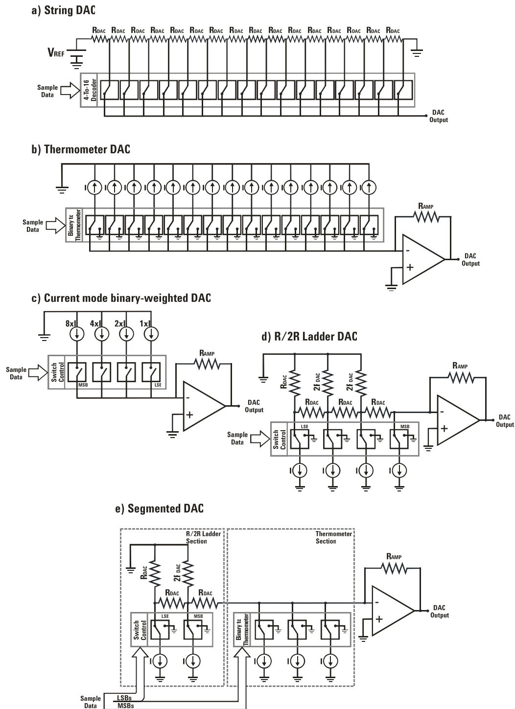
Figure 30: Different 4 bit DACs using the most popular DAC architectures. Unit-element based solutions are far more complex than binary-weighted ones, even for a limited vertical resolution. A trade-off between complexity, accuracy, and linearity leads to segmented DACs where some MSB are associated to a thermometer DAC section while the remaining LSBs are assigned to a binary-weighted DAC section.
