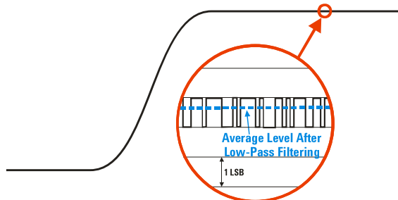
Figure 64: Dithering consist in adding a low level noise (1 LSBpp) to the waveform samples before quantization (a). In this way, any periodicity in the quantization noise will be removed (b) so the quantization noise will be spread out over a much larger number of
