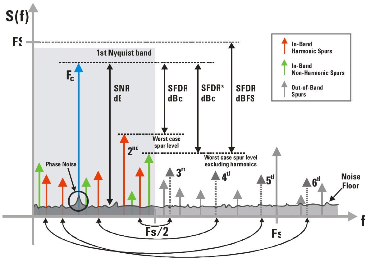
Figure 27: Non-linear behavior can be easily observed in the frequency domain by generating a pure sinewave. Nonlinearities result in unwanted components such as harmonics. Harmonics beyond the Nyquist frequency are folded down to the first Nyquist band. Other non-harmonic spurs may eventually show up in the spectrum. SFDR (Spurious-Free Dynamic Range) can be established through a spectrum analyser as well as noise floor and SNR (Signal-to-Noise Ratio).
