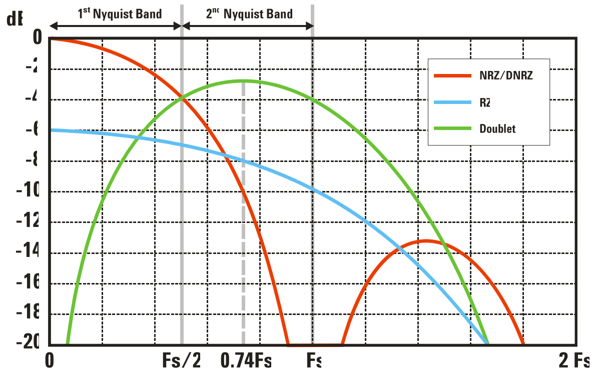
Figure 36: Frequency response for the four working modes in a dual-core architecture DAC. While the NRZ and RZ modes are mainly used to generate signals in the first Nyquist band, the Doublet mode enhances the response in the second Nyquist band making possible the generation of higher quality bandwidth-limited signals at higher frequencies.
