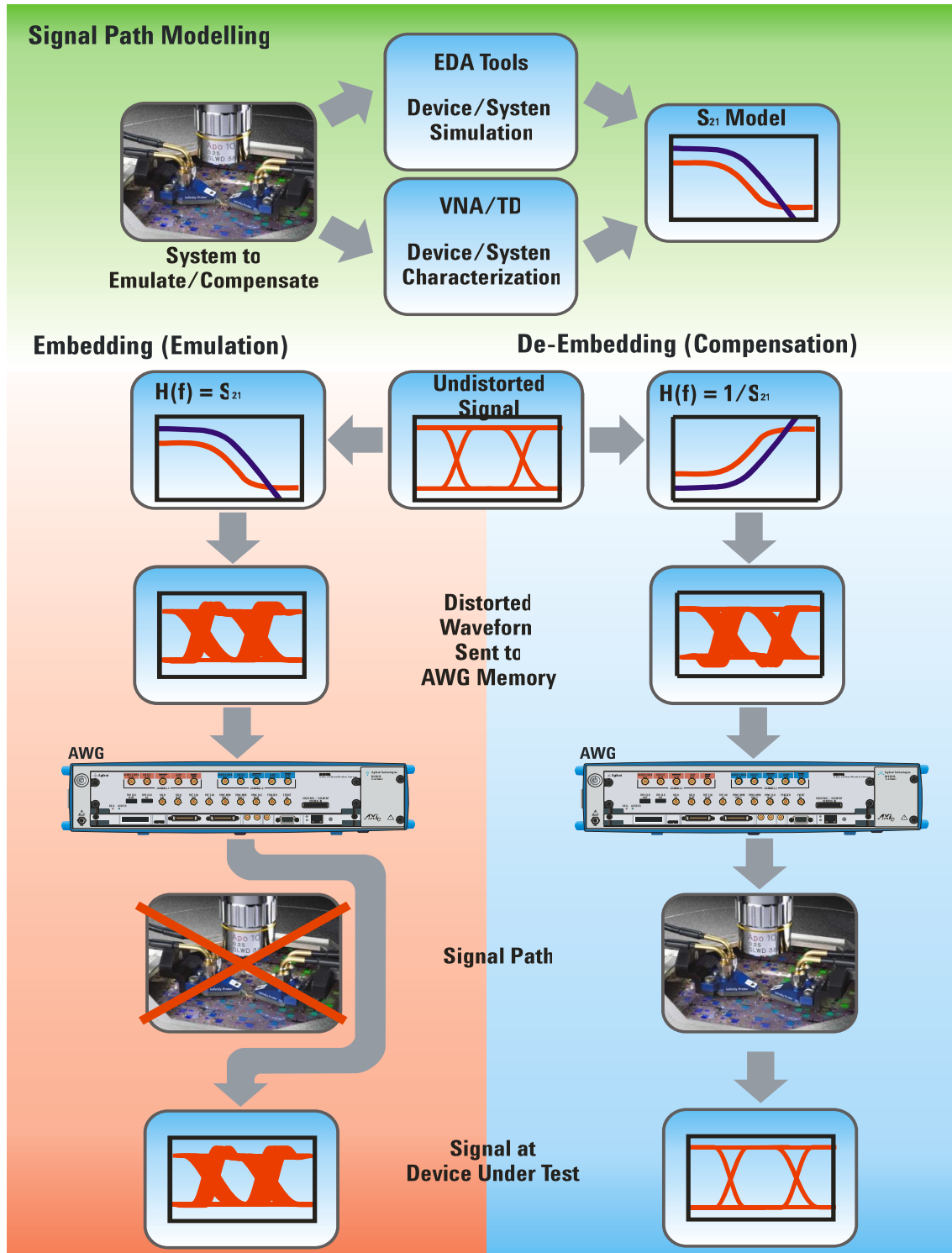
Figure 81: Embedding and de-embedding follow the same basic procedure. However, their goals are the opposite. Before application, an accurate model of the signal path (i.e. an interconnection in a PCB) must be obtained. Embedding applies the model to the undistorted signal so the effects of the modelled interconnection may be emulated. De-embedding applies a reversed response derived from the interconnection model so the signal at the end of the interconnection will be undistorted.
