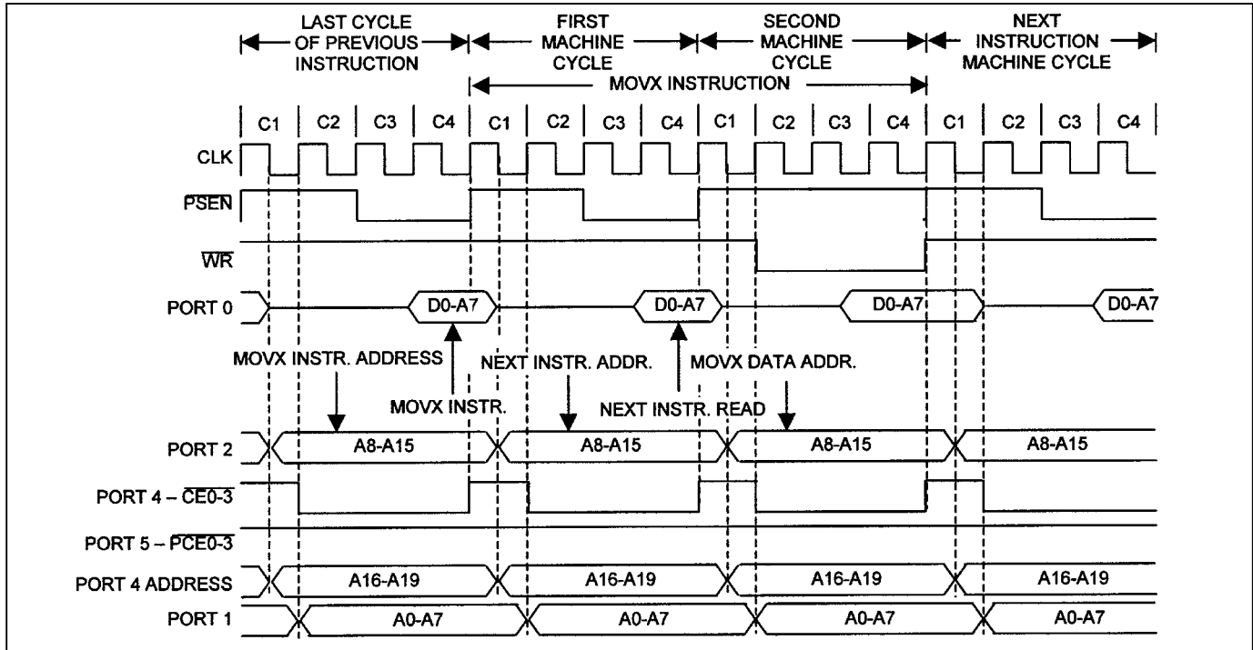
Figure 18. Nonmultiplexed 2-Cycle Data Memory \overline{\text{CE0-3}} Write
