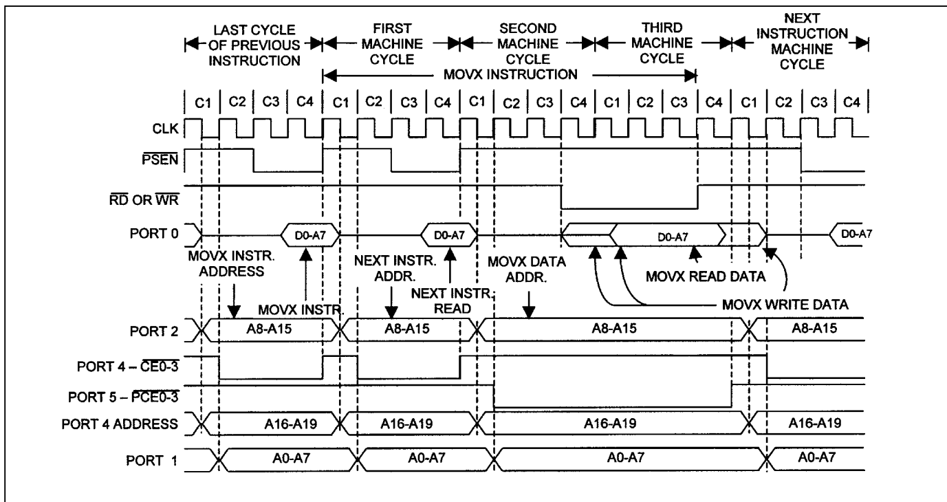
Figure 19. Nonmultiplexed 3-Cycle Data Memory \overline{\text{PE0-3}} Read or Write
