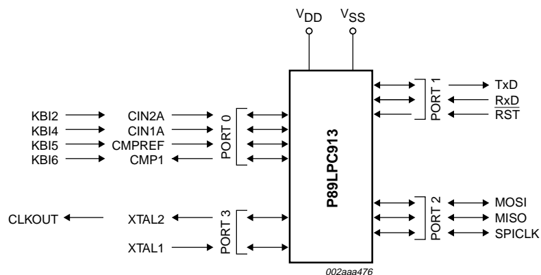
Fig 8. P89LPC913 logic symbol.
