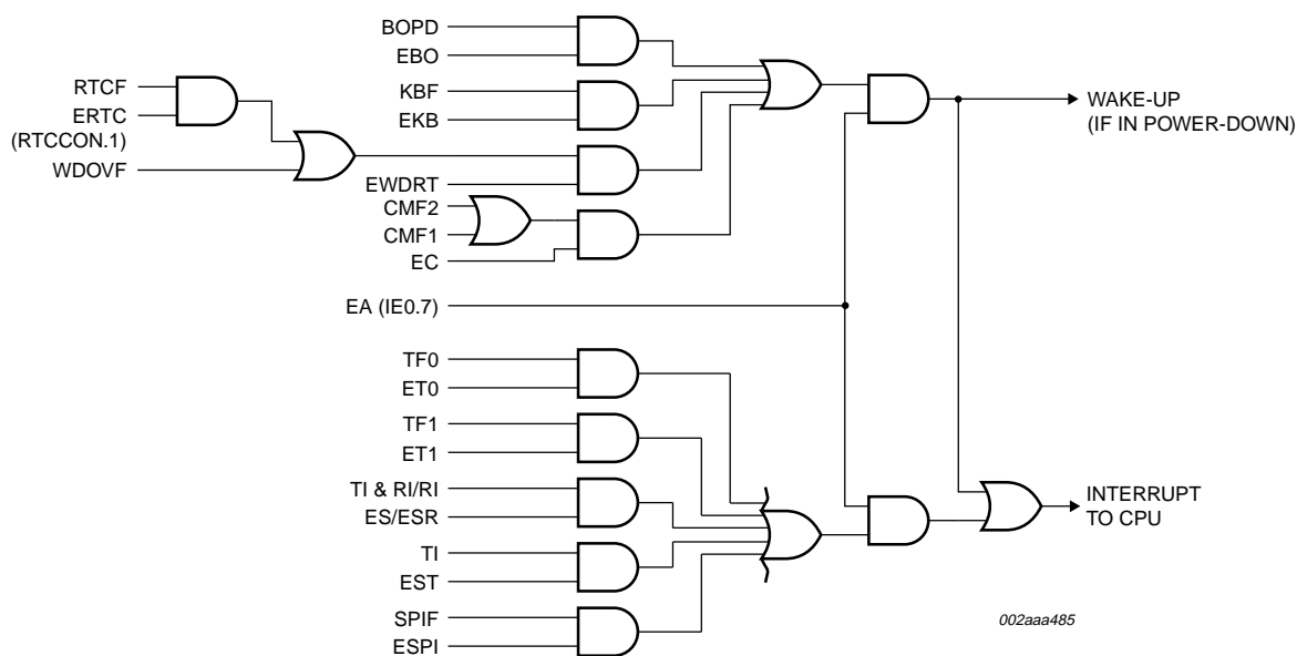
Fig 14. Interrupt sources, interrupt enables, and power-down wake-up sources (P89LPC913, P89LPC914).
