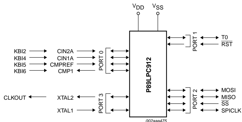
Fig 7. P89LPC912 logic symbol.
