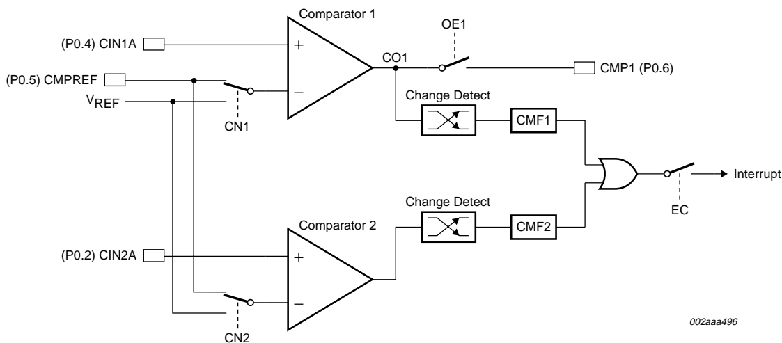
Fig 21. Comparator input and output connections.
