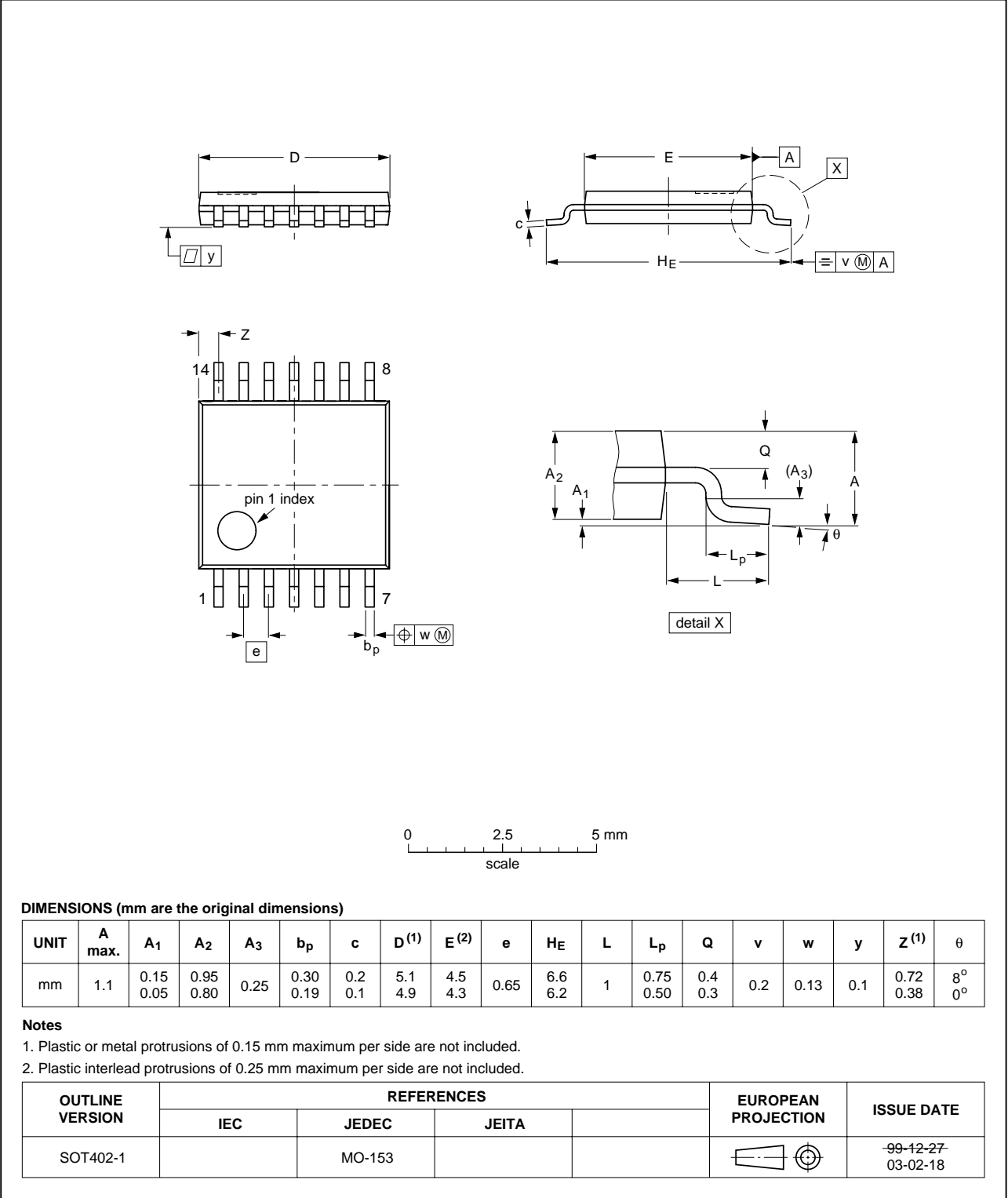
Fig 26. TSSOP14 package outline (SOT402-1).
