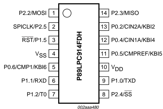
Fig 6. P89LPC914 TSSOP14 pin configuration.
