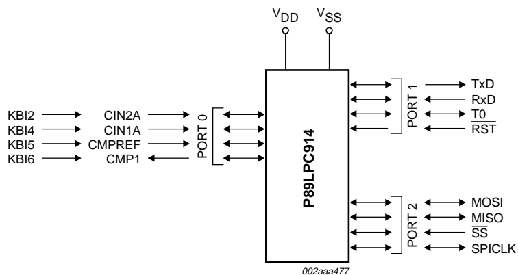
Fig 9. P89LPC914 logic symbol.
