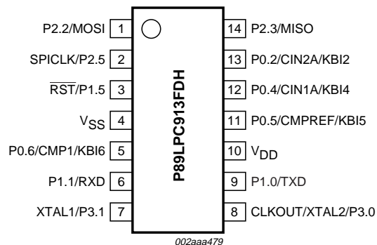
Fig 5. P89LPC913 TSSOP14 pin configuration.
