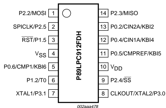
Fig 4. P89LPC912 TSSOP14 pin configuration.
