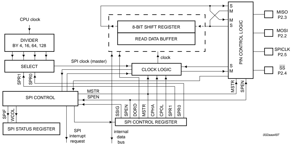
Fig 16. SPI block diagram (P89LPC912, P89LPC914).
