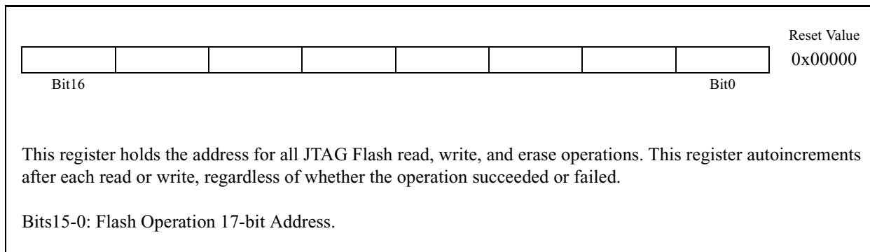
Figure 25.6. FLASHADR: JTAG Flash Address Register
