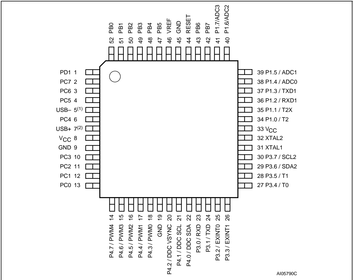
Figure 2. TQFP52 Connections
