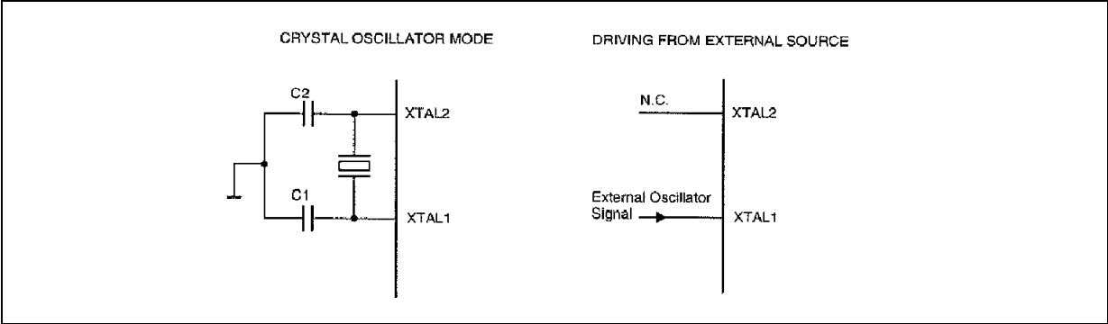
Figure 89. Recommended Oscillator Circuits
