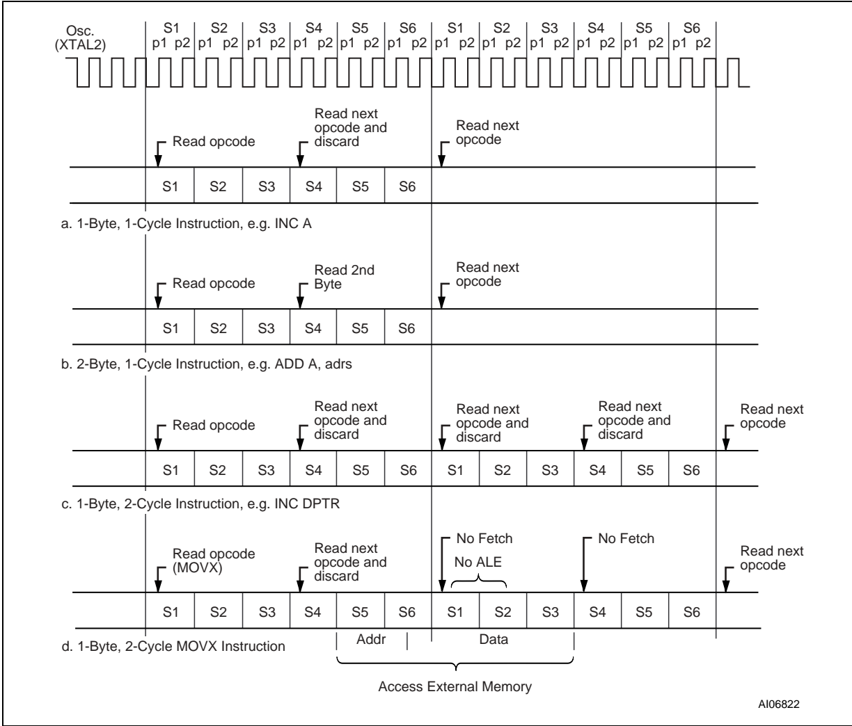
Figure 13. State Sequence in uPSD325X Devices
