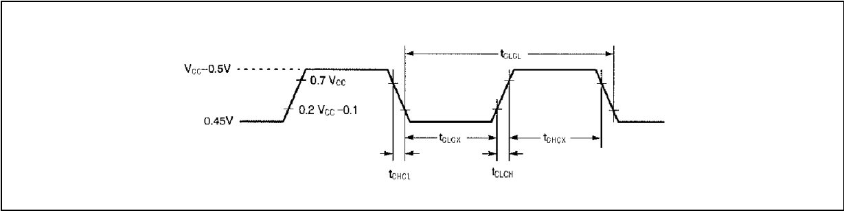
Figure 88. External Clock Cycle
