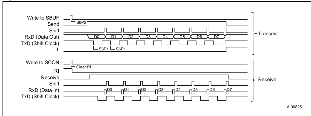
Figure 27. Serial Port Mode 0, Waveforms
