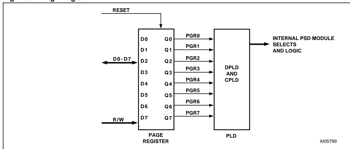
Figure 56. Page Register
