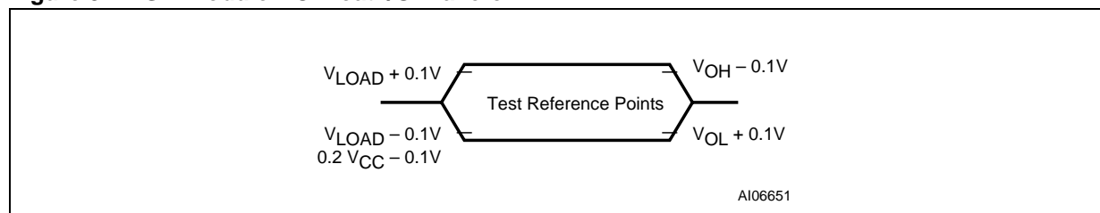
Figure 87. PSM Module AC Float I/O Waveform
