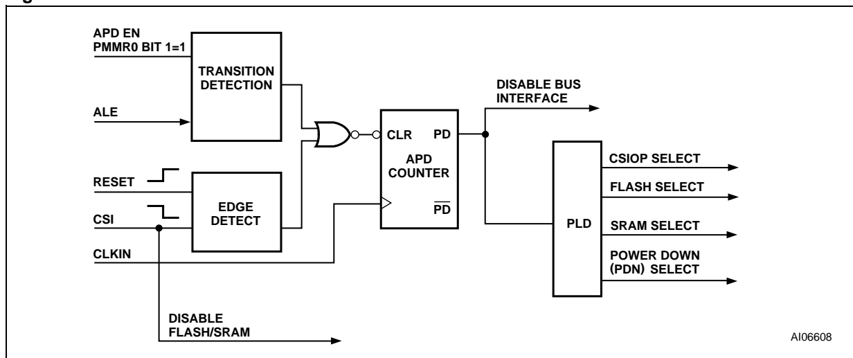
Figure 68. APD Unit
