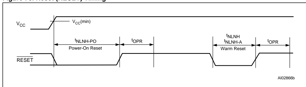
Figure 70. Reset ( \overline{\text{RESET}} ) Timing
