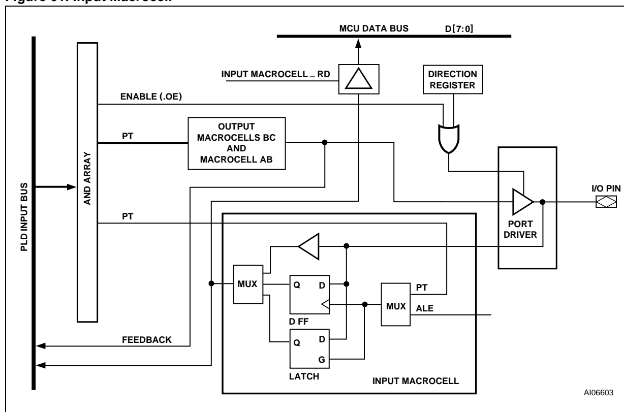
Figure 61. Input Macrocell
