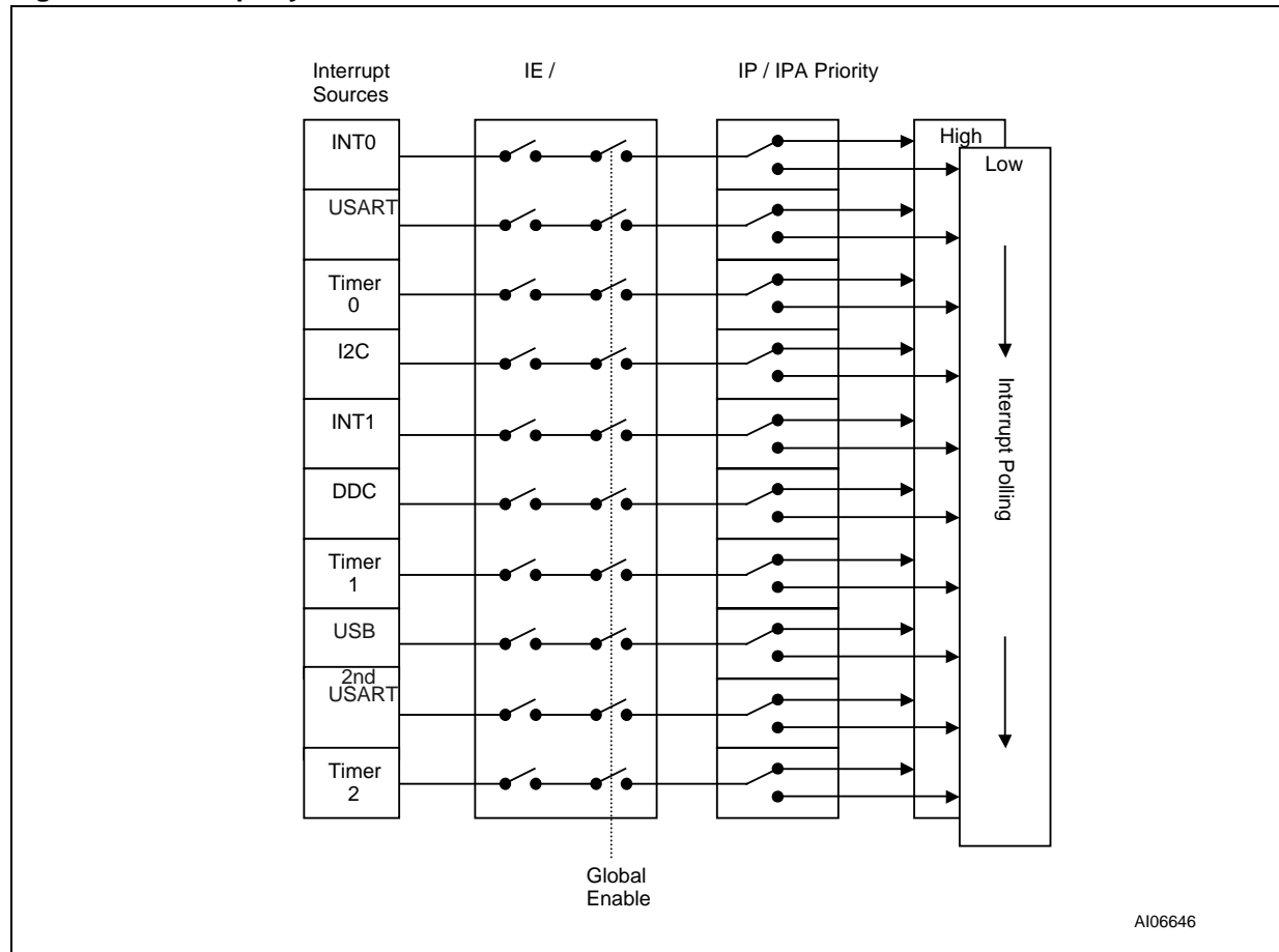
Figure 15. Interrupt System
