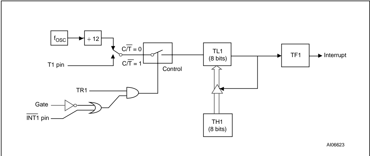
Figure 22. Timer/Counter Mode 2: 8-bit Auto-reload
