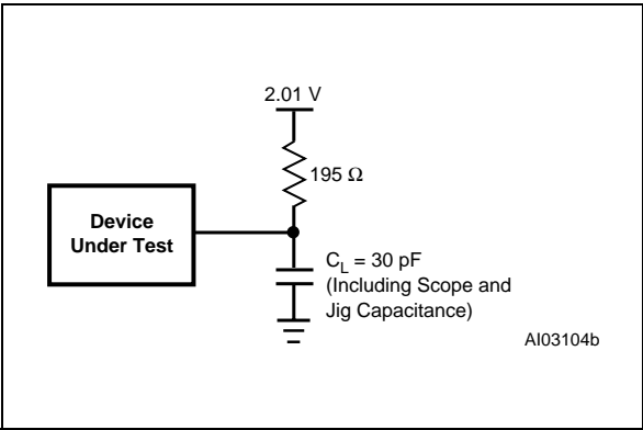
Figure 91. PSM Module AC Measurement Load Circuit
