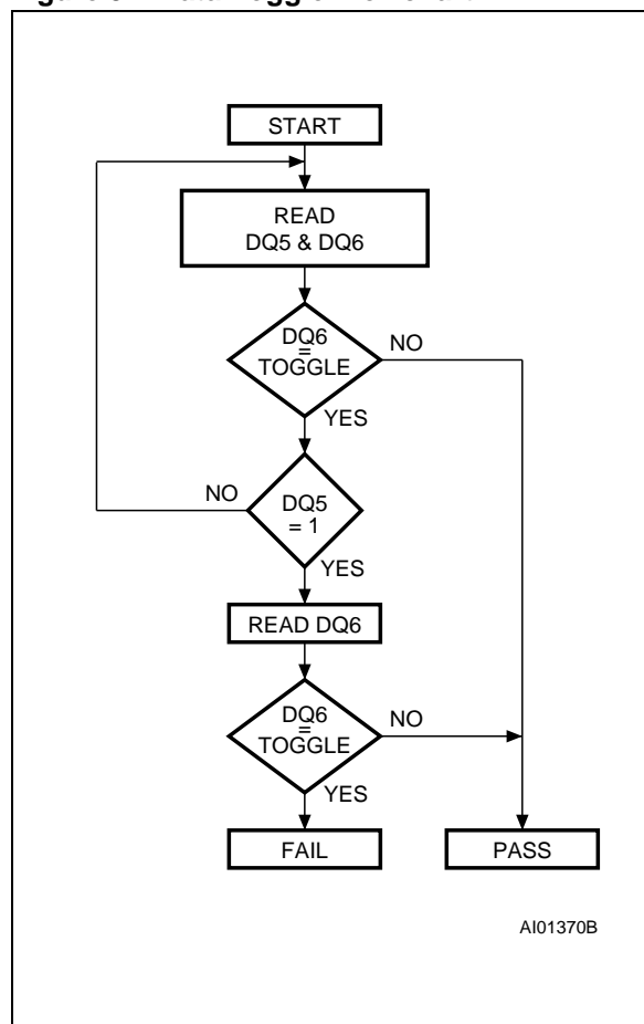
Figure 52. Data Toggle Flowchart
