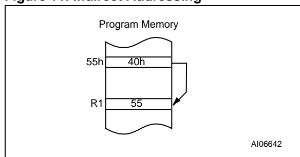
Figure 11. Indirect Addressing
