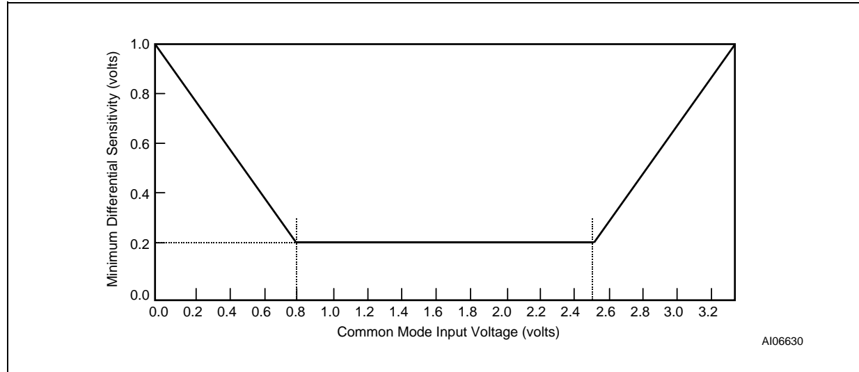
Figure 44. Differential Input Sensitivity Over Entire Common Mode Range
