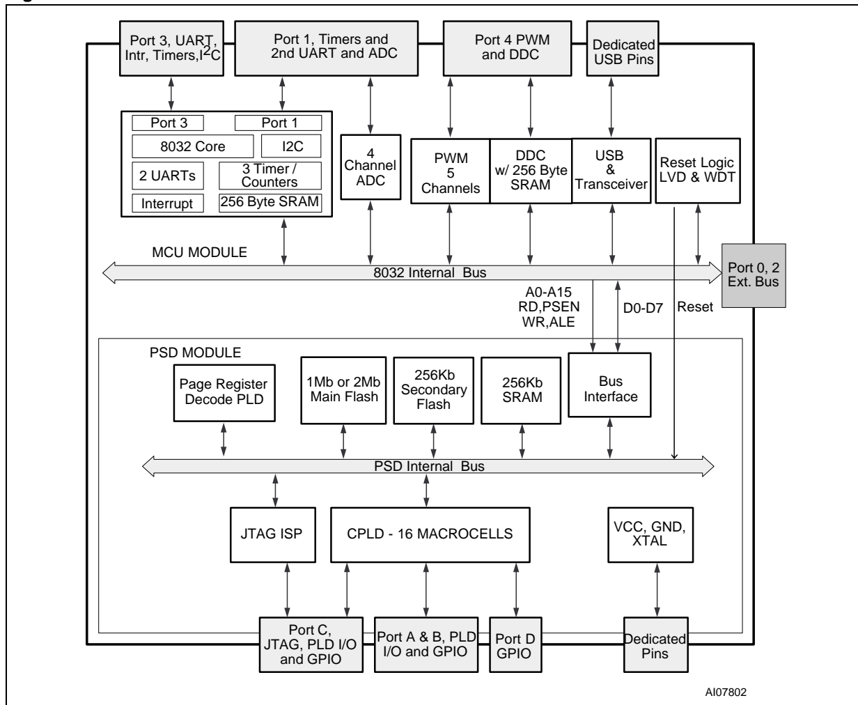
Figure 14. uPSD325X devices Functional Modules
