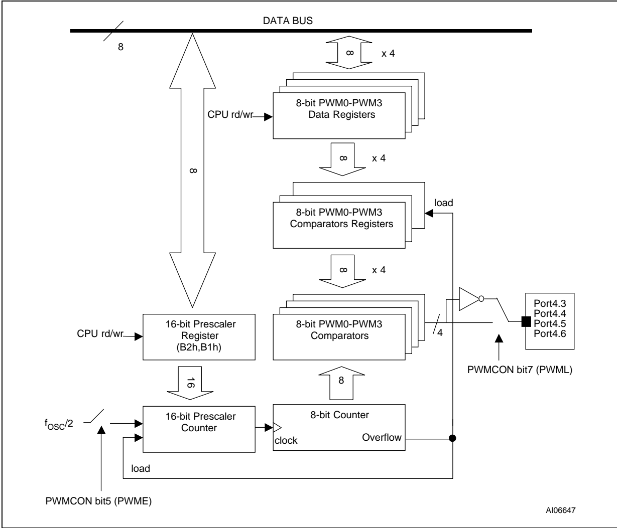
Figure 35. Four-Channel 8-bit PWM Block Diagram
