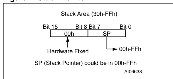
Figure 7. Stack Pointer
