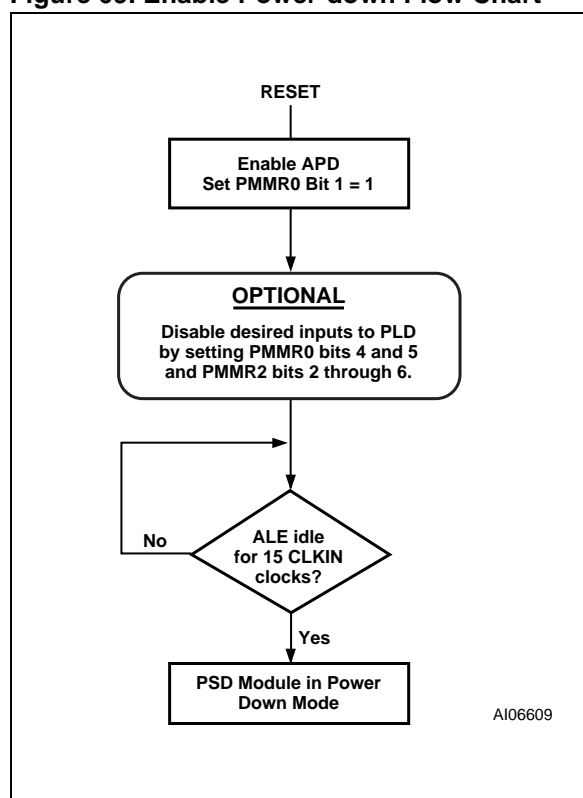
Figure 69. Enable Power-down Flow Chart
