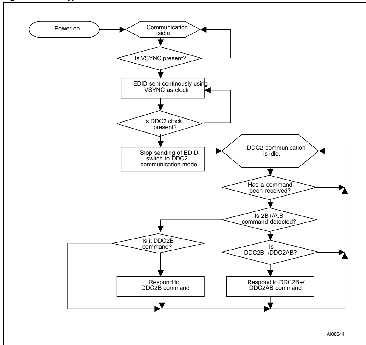
Figure 40. Host Type Detection
