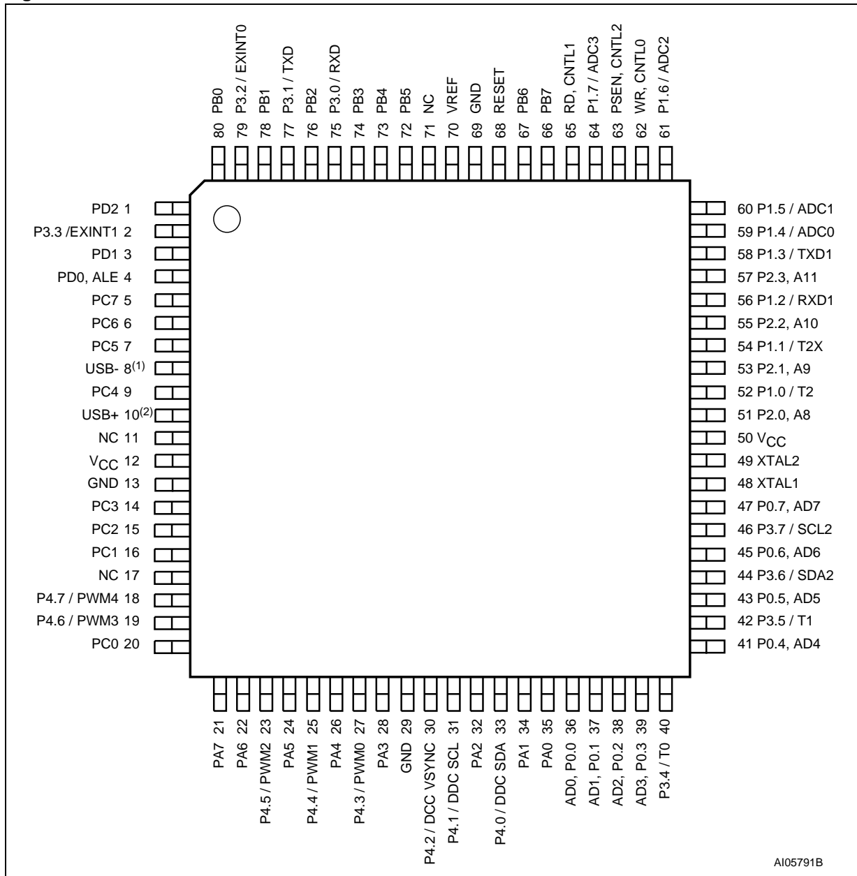
Figure 3. TQFP80 Connections
