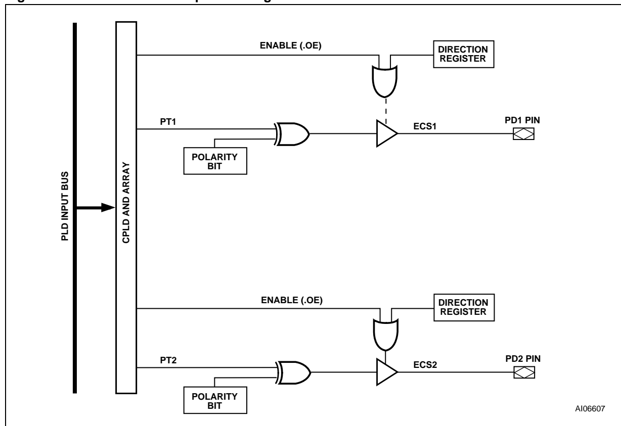
Figure 67. Port D External Chip Select Signals
