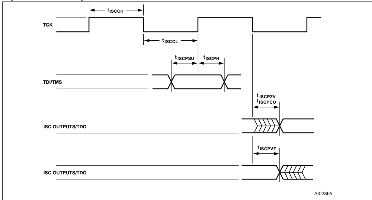
Figure 85. ISC Timing
