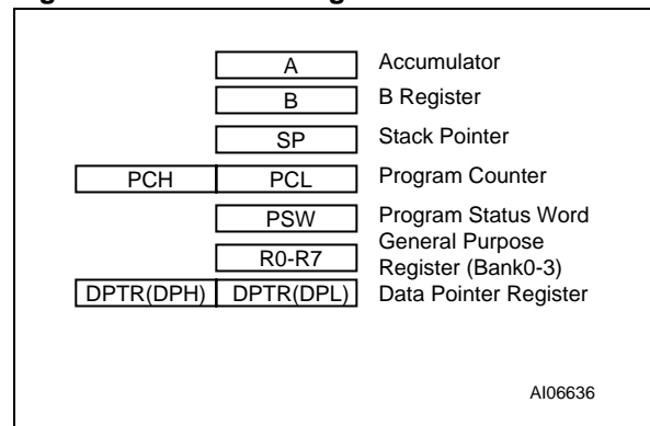
Figure 5. 8032 MCU Registers
