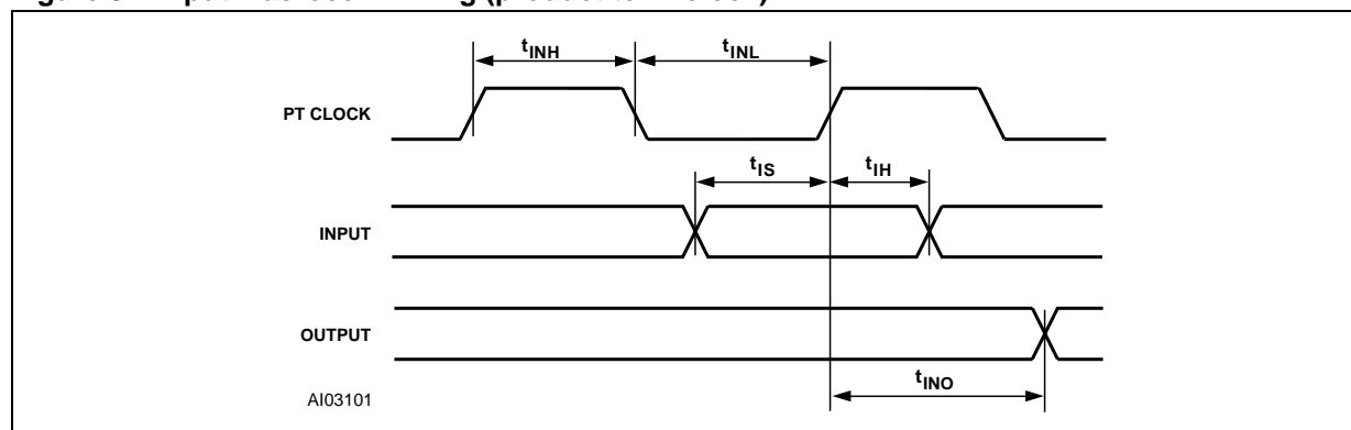
Figure 81. Input Macrocell Timing (product term clock)
