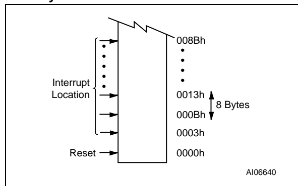
Figure 9. Interrupt Location of Program Memory
