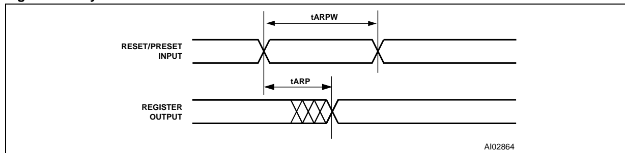
Figure 79. Asynchronous RESET / Preset
