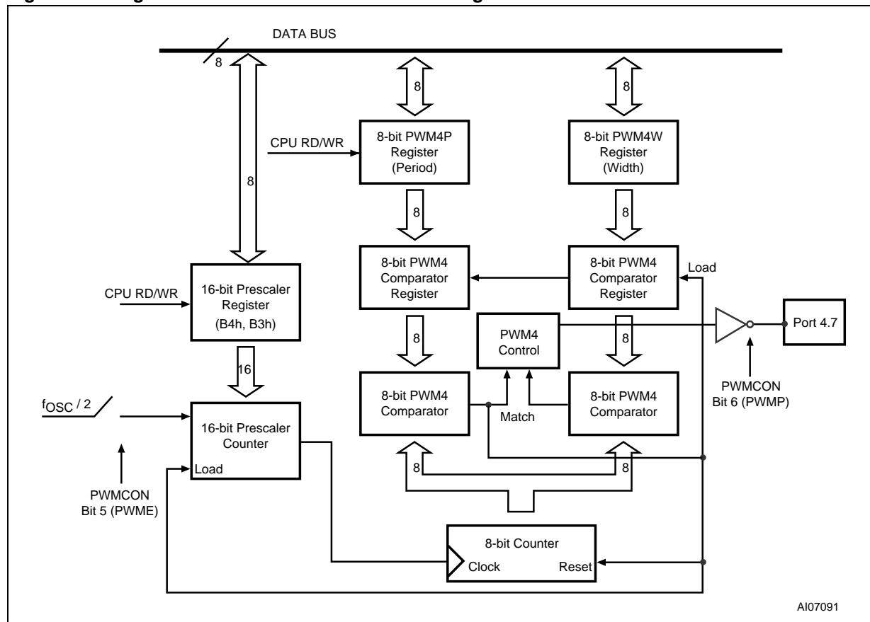
Figure 36. Programmable PWM 4 Channel Block Diagram
