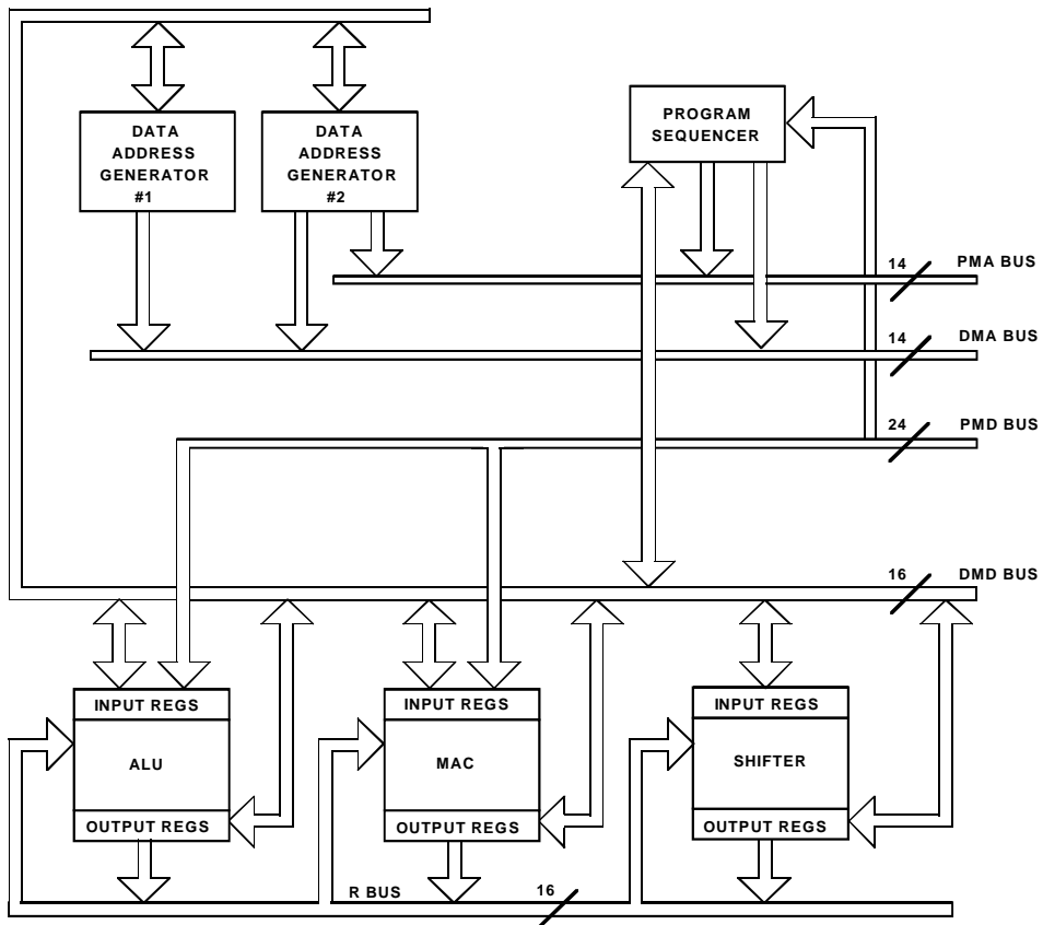
Figure 1-1. Core Architecture
